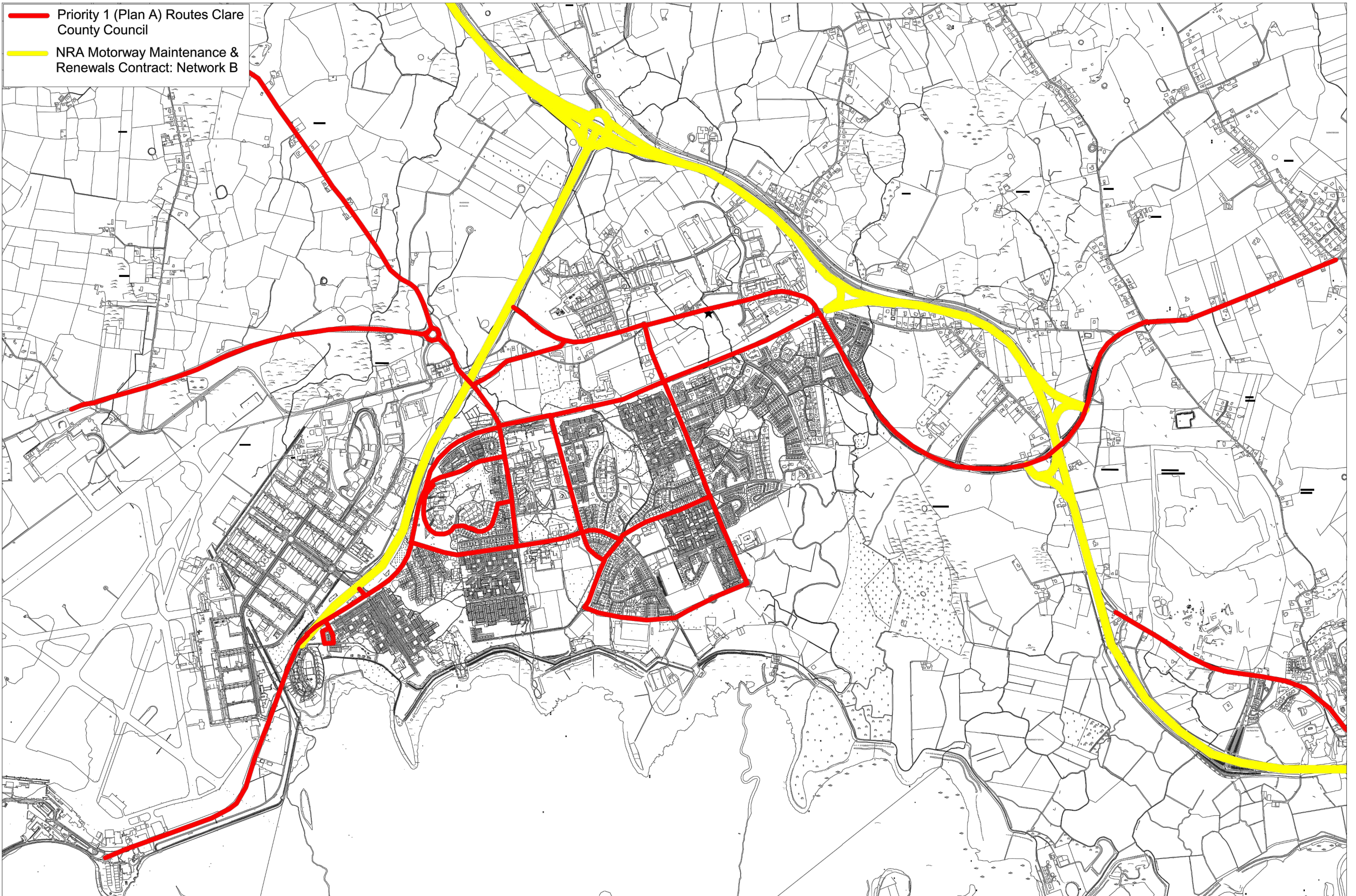
CLARE COUNTY COUNCIL - Salting Routes Winter Priority 1 (Plan A) Shannon Route
