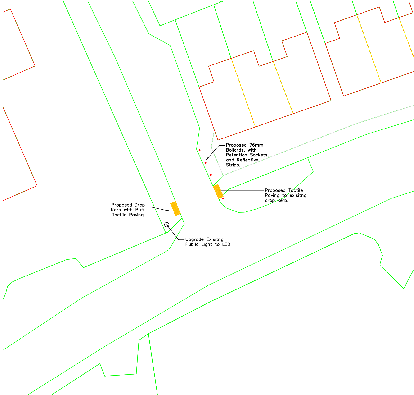
SITE LAYOUT PLAN Extract from O.S. 4090-D Scale: 1/250
